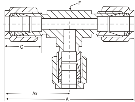
Dimensional Details :
