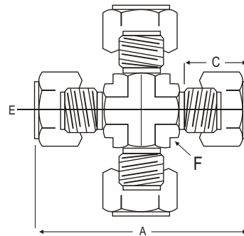
Dimensional Details :
